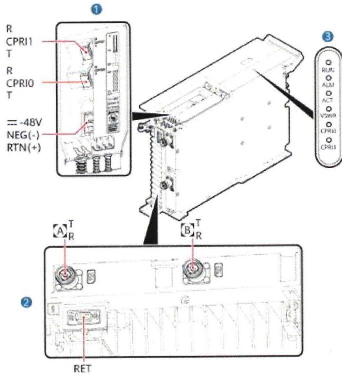
RRU5909(900M)
