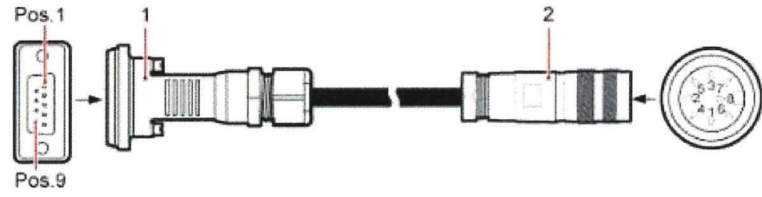
Figure 2 AISG multi-wire cable (2)
