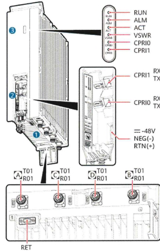
RRU5513(1800/2100M)
