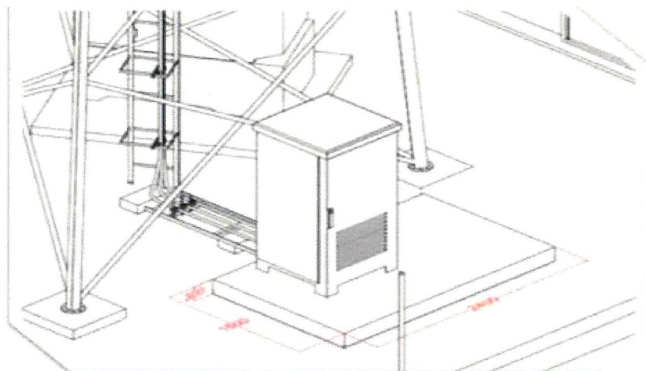
Single Cabinet – Standard Site
