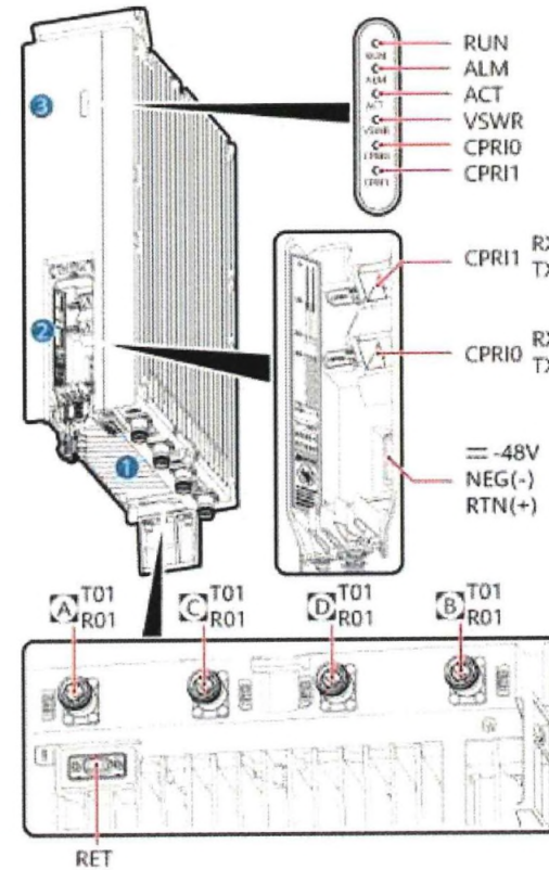
RRU5502(1800/2100M)
