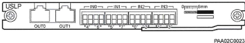
Figure 1 USLPc panel
