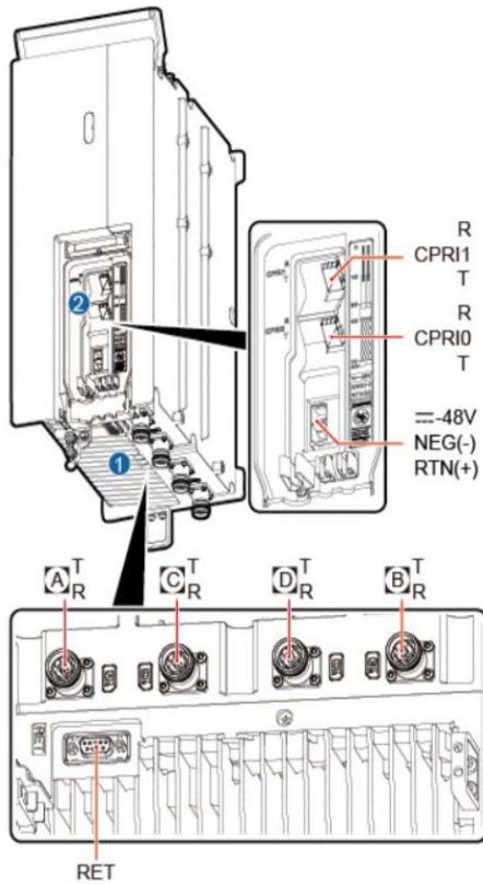
RRU5910(900M)
