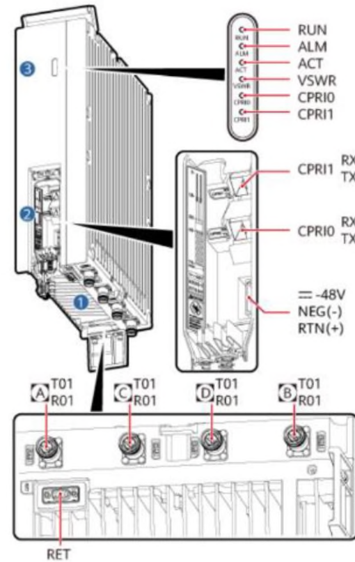
RRU5502(1800/2100M)
