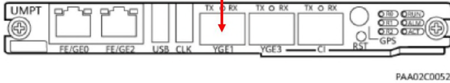
Figure 4 UMPTg panel
