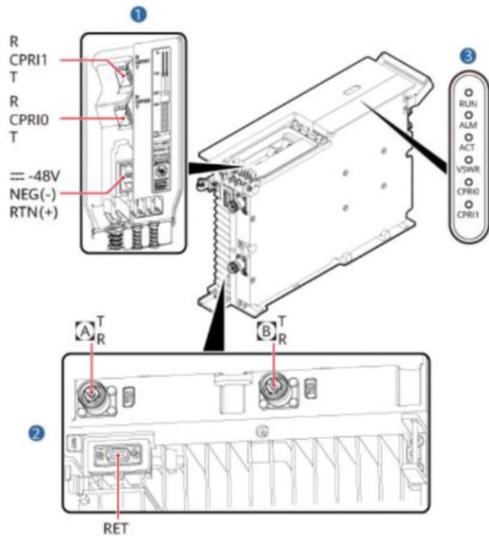
RRU5909(900M)
