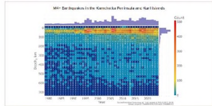
Fig. 75 Distribution of M4+ earthquakes recorded in the selected sector of the Kamchatka Peninsula and Kuril Islands region from 1979 to 2024 by depth. Data source: ISC.
